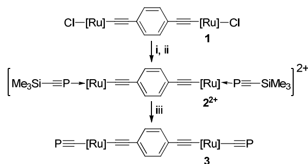
Scheme 1: Reagents and conditions: i) \text{CH}_2\text{Cl}_2 , 2 \text{AgOTf} , ii) 2 \text{P}\equiv\text{CSiMe}_3 in toluene, 1h.; iii) \text{thf} , 2 \text{KO}^t\text{Bu} , 1h. [\text{Ru}] = \text{Ru}(\text{dppe})_2 .
