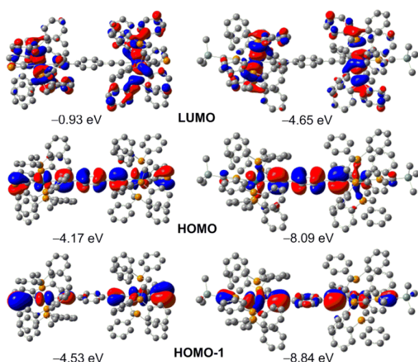
Figure 2: Frontier orbitals for 3 (left) and 2 2+ (right), with relative energies (see also ESI).
