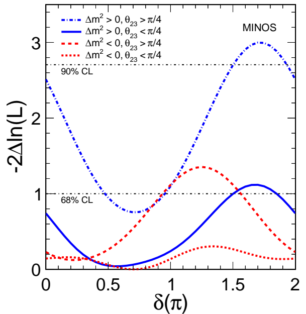
FIG. 4: The resulting values of the likelihood L , shown here as -2\Delta\ln L , from a fit of \delta to our data using constraints from reactor experiments [8–10], assuming various values of the mass hierarchy and the sign of \theta_{23} - \pi/4 . The difference is taken with respect to the best-fitting solution. Values above the horizontal dashed lines are disfavored at either 68% or 90% C.L.
