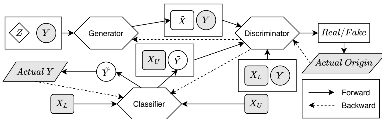
Figure 1: This network was used in the classification process. Dashed backward lines represent target variables, which are compared against predicted ones to perform gradient descent. The discriminator is trained to distinguish between real data-label pairs originating from the training data and fake data, which includes synthetic data created by the generator and unlabelled data with predicted labels. The discriminator serves as adversarial for the other networks, guiding the generator to create more realistic samples and the classifier to predict more accurate labels. A detailed description can be found in Sec. 3.
