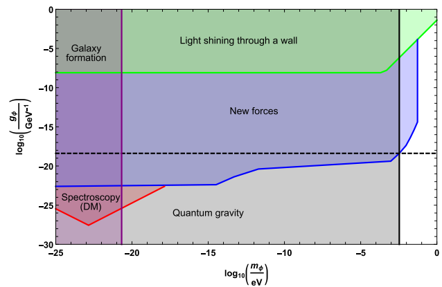
Fig. 1 Limits on the linear scalar interaction g_\phi = c_1/\Lambda_1 as a function of the mass of the scalar m_\phi . Green: limits from light shining through a wall experiments [46,47]. Blue: limits from torsion experiments [34–42]. Red: limits from atomic spectroscopy experiments [43–45]. Purple: limits from galaxy formation, quasar lensing and stellar streams [48–53]. Black: limits from quantum gravity as discussed in this paper. Dashed black line: reduced Planck scale
