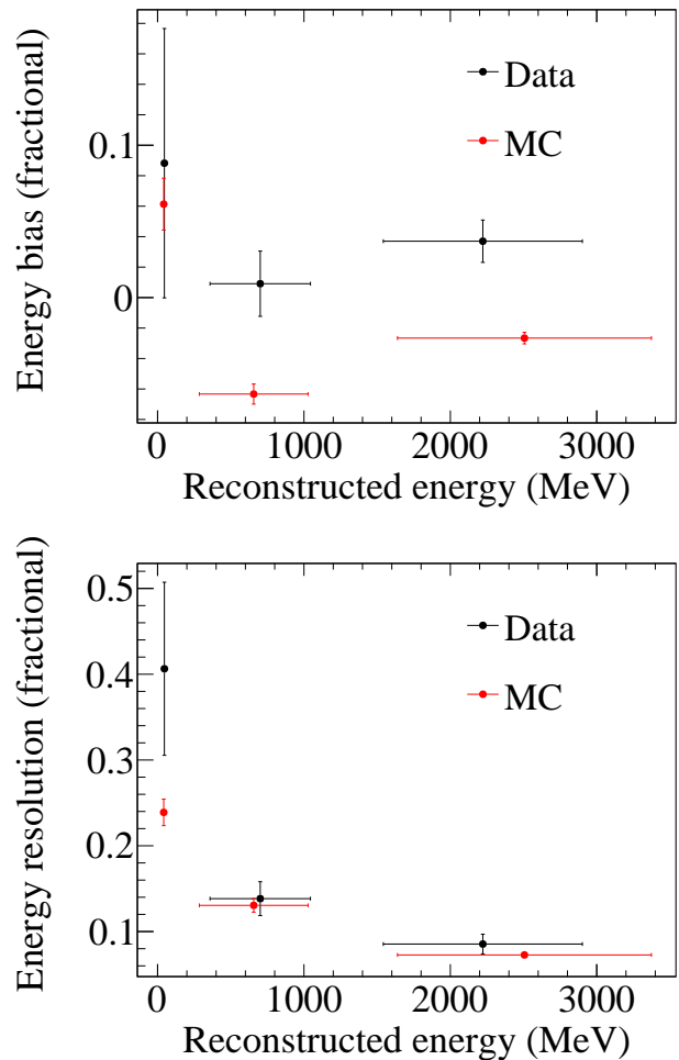
FIG. 12. Energy bias (top) and resolution (bottom) derived from the Michel electron (first point on the left) and stopping muon control samples (two last points on the right).
