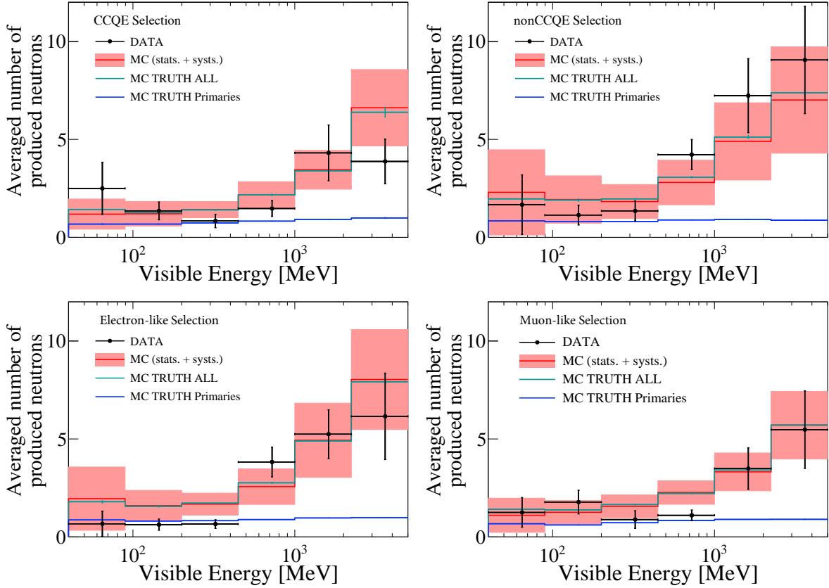
FIG. 15. Averaged number of produced neutrons versus visible energy for both phases together. We show the different selections: CCQE (top-left), nonCCQE (top-right), electron-like (bottom-left) and muon-like (bottom-right). The points represent data with statistical uncertainties. The reconstructed MC is shown with red boxes with the size corresponding to the systematic uncertainties. The green line represents the average total number of neutrons given by the MC truth and the blue line corresponds to the average number of primary neutrons given by the MC truth.
