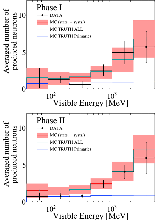
FIG. 14. Averaged number of produced neutrons versus visible energy for Phase I (top) and Phase II (bottom). The points represent data with statistical uncertainties. The reconstructed MC is shown with red boxes with the size corresponding to the systematic uncertainties. The green line represents the average total number of neutrons given by the MC truth and the blue line corresponds to the average number of primary neutrons given by the MC truth.
