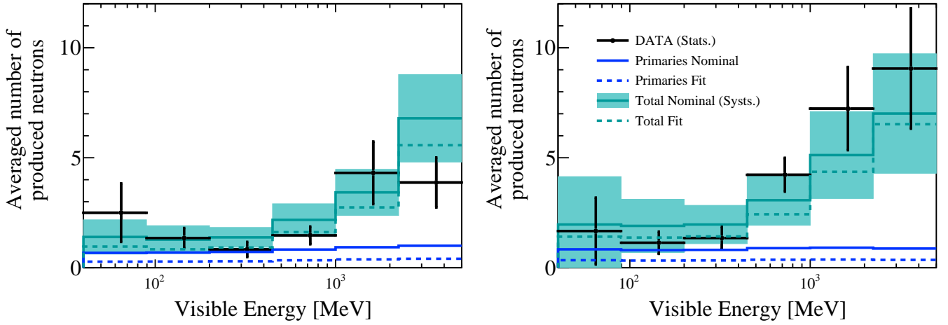
FIG. 18. Number of produced neutrons versus visible energy for CCQE (left) and nonCCQE (right) selections before and after \chi^2 fit to neutron components. This combines both phases.
