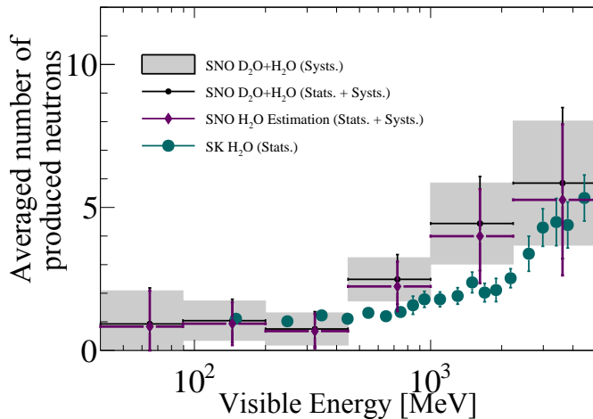
FIG. 17. Neutron production measurement in this work compared to SK published results [8]. Black dots correspond to the present work, with grey boxes representing systematic uncertainties and solid lines being the total uncertainties. The estimation of SNO with pure light water (see text for details) is shown with diamonds. The nominal SK measurement with light water is marked with circles and it only displays statistical uncertainties.
