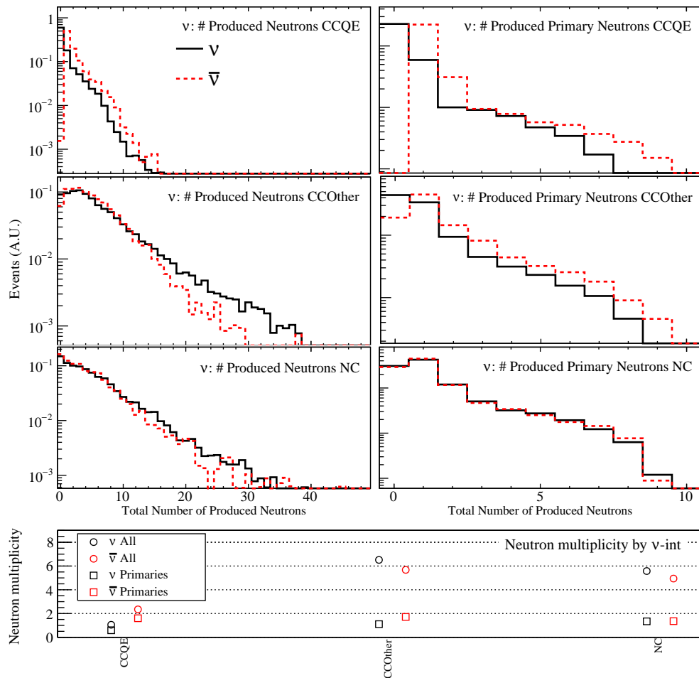
FIG. 3. Predicted neutron production in the SNO detector per event for different neutrino interactions (rows) with no event selection applied. Total neutron production is shown on the left and only primary neutrons on the right. At the bottom, the average number of neutrons are shown for each case.
