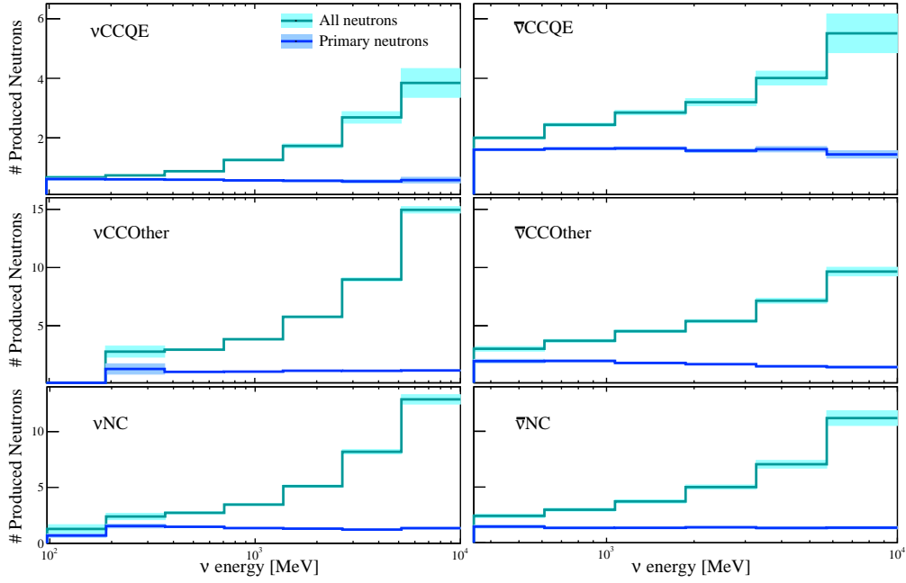
FIG. 4. Predicted neutron production in the SNO detector as a function of the neutrino energy for different neutrino interactions and for neutrinos (left) and anti-neutrinos (right). No event selection is applied.
