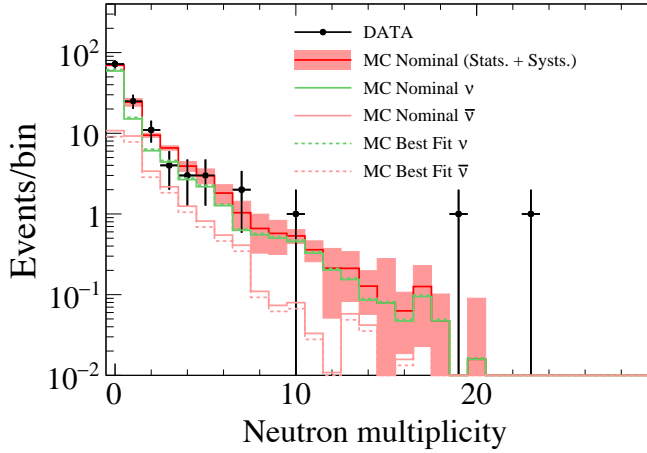
FIG. 19. Number of detected neutrons per neutrino interaction candidate in both phases. The MC shows the systematic uncertainties and it is broken down into \nu and \bar{\nu} . The fit results are also shown.
