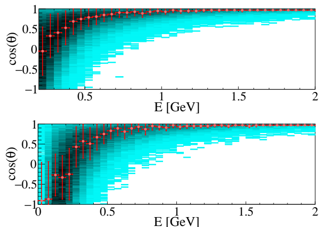
FIG. 5. Angle of produced lepton \cos \theta_l versus lepton energy in a CCQE neutrino interaction for muons (top) and electrons (bottom). The red dots show the mode of the \cos \theta distribution at each energy bin with the 1\sigma uncertainty.
