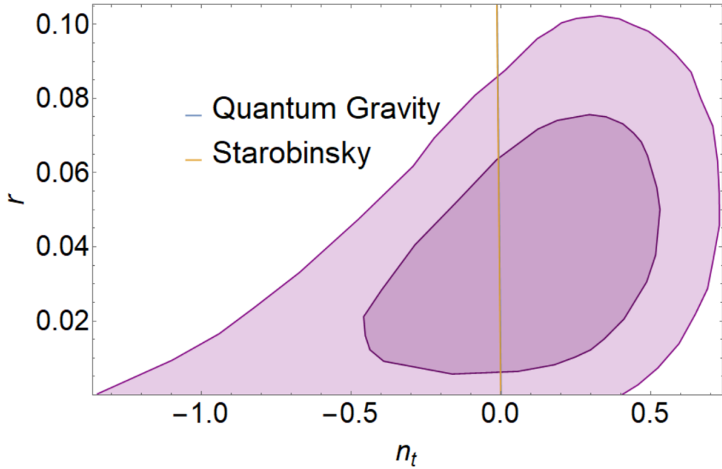
Figure 1: We plot the tensor-scalar ratio r against the tensor spectral tilt n_t for Starobinsky inflation and Effective Quantum Gravity, using (25) and choosing m_2/H = 0.001 , against the 2018 Planck results [17]. The line for Starobinsky’s model (orange line) overlaps the blue line corresponding to Quantum Gravity precisely, making it impossible to distinguish between both lines with current data.
