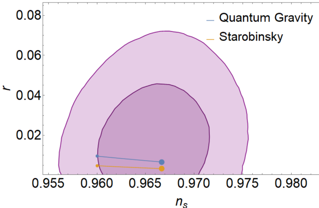
Figure 2: We plot the tensor-scalar ratio r against the scalar spectral tilt n_s for Starobinsky inflation and Effective Quantum Gravity, using (9) and (24), against the 2018 Planck results [17]. The small dot represents N = 50 e-folds and the large dot represents N = 60 .
