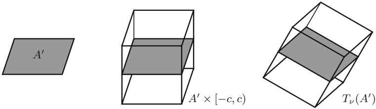
Fig. 1. Construction of the oriented n -dimensional interval T_\nu(A')
