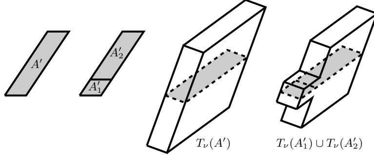
FIGURE 2. An example with N = 2 in which T_\nu(A') \neq T_\nu(A'_1) \cup T_\nu(A'_2) .
