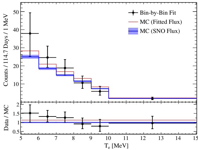
FIG. 3. Top: The extracted solar neutrino elastic scattering event rate as a function of reconstructed electron kinetic energy T_e . Bottom: The same, as a fraction of the expected rate. The red and blue lines show the MC simulation predicted spectrum normalized to the best fit flux and the SNO flux measurement [28], respectively. The uncertainty on the SNO result includes reported uncertainty combined with mixing parameter uncertainties. The black points are the results of the fits to the \cos\theta_{\text{sun}} distribution in each energy bin, with error bars indicating the combined statistical and systematic uncertainty, including energy-correlated uncertainty. A horizontal dash is placed on each error bar, indicating the statistics only uncertainty; for all points the statistical error is dominant and the systematic error bar is not visible above the dash.
