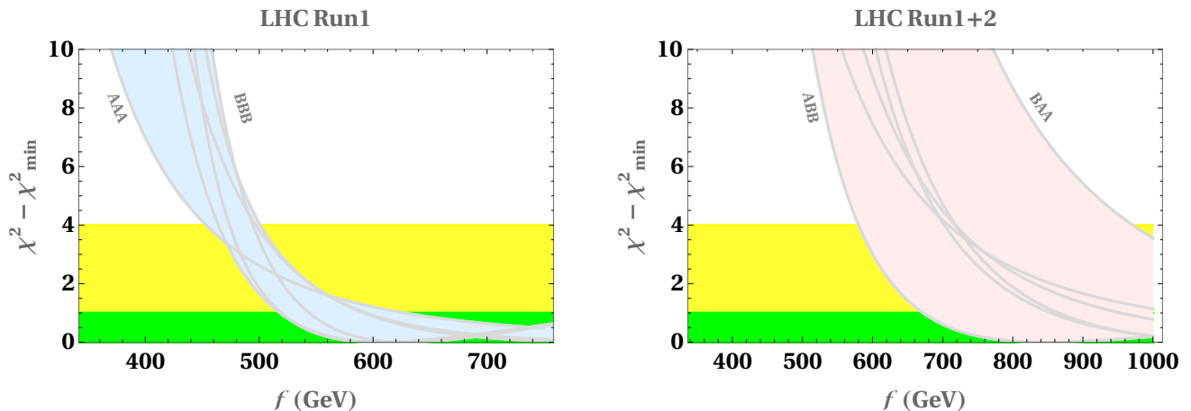
FIG. 1: \chi(f)^2 - \chi_{min}^2 for the Run 1 (left) and combination of Run 1 and 2 (right) datasets. The lines correspond to different choices of fermion couplings \kappa_F^{A,B} for (\kappa_t, \kappa_b, \kappa_\tau) . For example, AAA indicates \kappa_t = \kappa_b = \kappa_\tau = \kappa_F^A .
