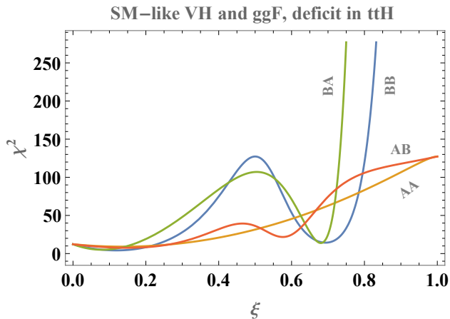
FIG. 2: \chi(\xi)^2 assuming a scenario where a deficit is found in ttH production channels, while other channels remain consistent with the SM. The labels correspond to different hypothesis of \kappa_F^{A,B} for (\kappa_t, \kappa_b) . In this case, the choice \kappa_t = \kappa_b = \kappa_F^B would be preferred by data. We assume a 20% uncertainty in these channels, except in gg \rightarrow H \rightarrow \gamma\gamma where a 10% accuracy is assumed.
