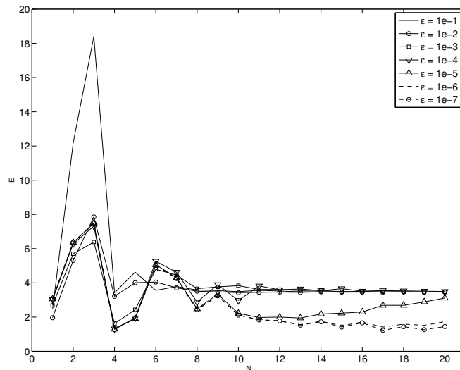
(a) Effectivities for varying \varepsilon .
