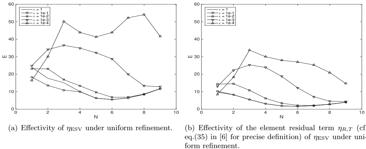
FIGURE 6. Effectivity of estimator under uniform refinement.
