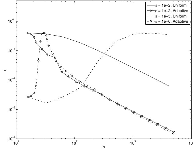
(b) Error convergence under uniform and adaptive refinement.
