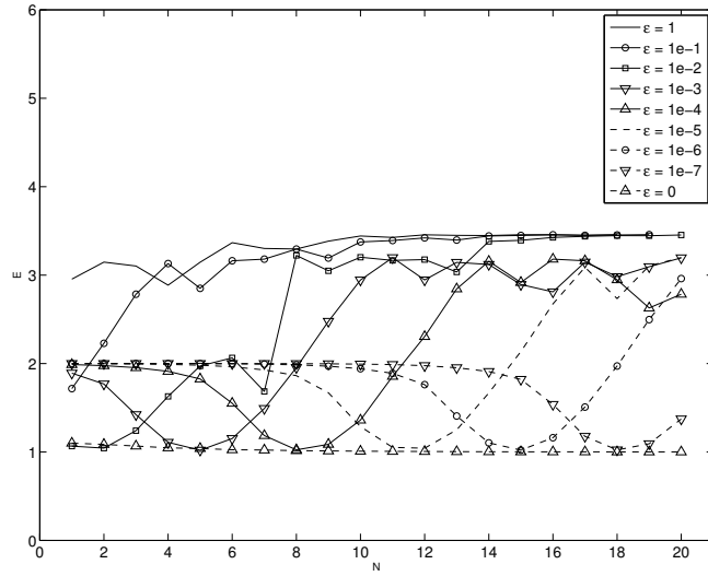
(a) Effectivity of the error estimator.
