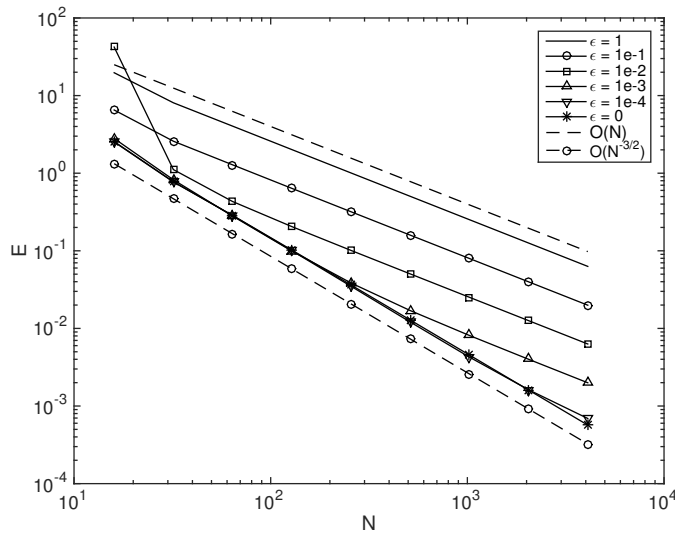
(a) Error convergence under uniform refinement.
