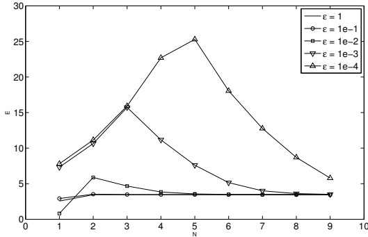
(b) Contribution of residual term, \eta_R .
