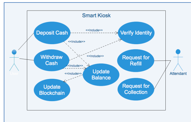
Figure 1: Smart Kiosk Use Case Diagram
