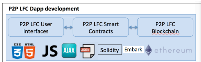
Figure 3: P2P LFC Exchange Architecture
