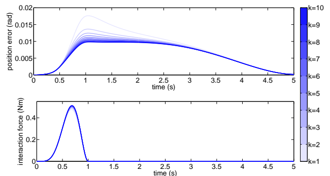
Fig. 4. Position errors and interaction forces in the first case
