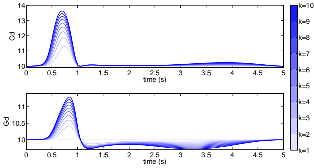
Fig. 5. Damping and stiffness parameters in the first case
