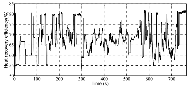
Fig. 9 Heat recovery efficiency over entire operating period
