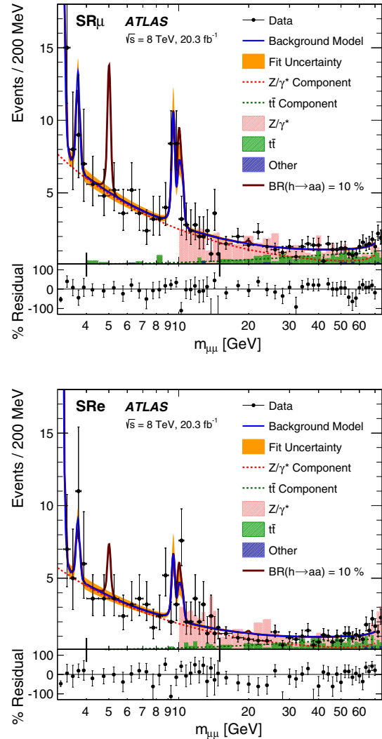
FIG. 4 (color online). Observed m_{\mu\mu} distribution in SR_\mu (top) and SRe (bottom) and the background-only fit. The Z/\gamma^* component of the fit is the combination of the Z boson resonance and the \gamma^* continuum models. The % residuals are shown below each plot. Bins below 4 GeV are 200 MeV wide, between 4 GeV and 15 GeV they are 500 MeV wide, and above 15 GeV they are 2 GeV wide. The expected distribution from a signal with BR(h \rightarrow aa) = 10\% is shown for three different m_a hypotheses (5, 10, and 20 GeV). Simulated SM backgrounds are shown in the stack, with the Z/\gamma^* sample only valid above m_{\mu\mu} > 10 GeV.
