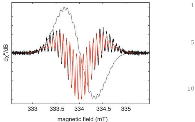
Fig. 2 X-band first (grey dotted line) and second (solid black line) derivative ESR spectrum of 3 at room temperature in benzene solution. A simulation of the second derivative spectrum is shown in red. Instrumental parameters: \nu = 9.379 \text{ GHz} , modulation frequency = 100 \text{ kHz} , modulation amplitude = 0.1 \text{ G} , microwave power = 0.25 \text{ mW} , conversion time = 40 \text{ ms} , 4 scans.
