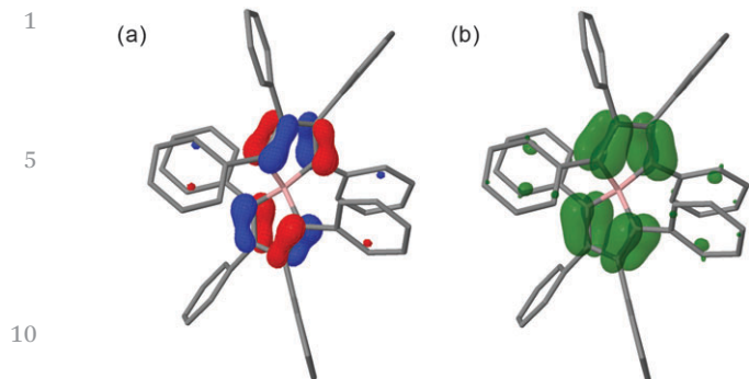
Fig. 3 MO62X/6-311G* calculated (a) singly-occupied molecular orbital (SOMO), and (b) spin-density distribution for 3 with imposed D_2 symmetry.
