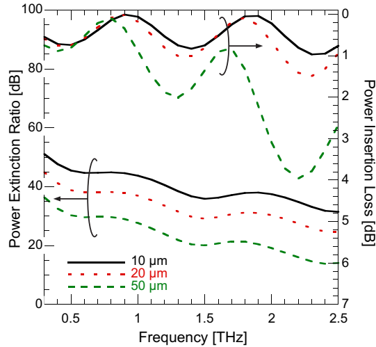
Fig. 2. Numerical investigation of the ER and IL of the THz WGP at normal incidence for a pitch fill factor F = 70\% as a function of the pitch on a 100\ \mu\text{m} -thick foil.
