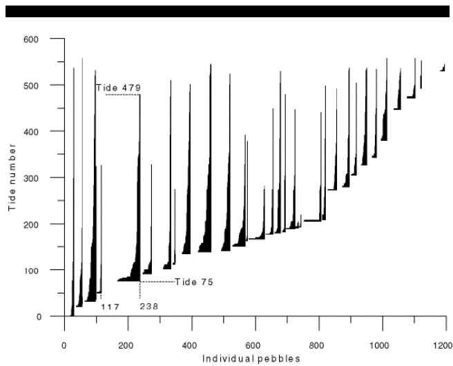
Figure 4. Summary of pebble seeding times and collection times. Column height represent the amount of time a particular pebble has spent on the beach between seeding and collection. Gaps indicate pebbles that have been seeded but not yet recovered. Of all the pebbles put out at tide 75 (pebble 117 to 238), for example, 49 are still on the beach indicated by the gap and two pebbles (at 237 and 238) have been recovered after 404 tides (between tide 75 and 479) indicated by the very long column.
