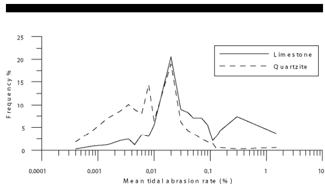
Figure 5. Frequency graph for 681 pebble records with abrasion rate >0%.
