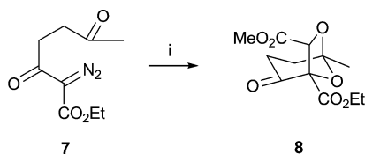
Scheme 2 Reagents and conditions: methyl glyoxylate, \text{Rh}_2(\text{OAc})_4 (cat.), PhMe, 110 °C (60%). 10,11
