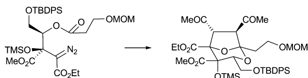
Scheme 3 Reagents and conditions: ( E )-3-hexene-2,5-dione, \text{Rh}_2(\text{OAc})_4 (cat.), benzene, 80 °C (47%). 12
