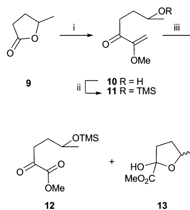
Scheme 4 Reagents and conditions: i, methyl vinyl ether, t -BuLi, THF, –78 °C (92%); ii, TMSCl, pyridine, THF, 0 °C, (92%); iii, \text{O}_3 , \text{CH}_2\text{Cl}_2 , –78 °C, then \text{Ph}_3\text{P} ( 12 : 33% and 13 : 30%).
