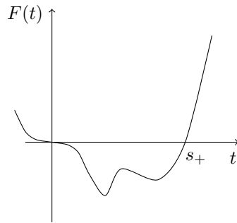
FIG. 1. A graph of a prototypical nonlinearity F .
