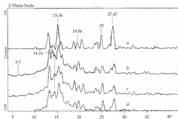
Fig. 2. XRPD patterns of carbamazepine crystals: a) untreated carbamazepine and that grown in media with pH: b) 1, c) 7 or d) 11.
