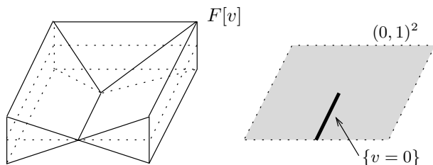
FIGURE 1.3. A polyhedron in \mathbb{R}^3 such that the rigidity condition (1.6) and the “no vertical parts” condition hold (with \Omega = (0, 1)^2 ), but such that the “no vanishing sections” condition fails.
