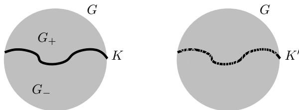
FIGURE 1.4. In the picture on the left, G is a disk and K is a smooth curve that divides G in two open regions G_+ and G_- , in such a way that (1.8) holds: thus, K essentially disconnects G . Let now K' be obtained by removing some points from K . If we remove a set of length zero, that is, if \mathcal{H}^1(K \setminus K') = 0 , then K' still essentially disconnects G (although G \setminus K' may be easily topologically connected!); if, instead, \mathcal{H}^1(K \setminus K') > 0 , then K' does not essentially disconnect G , since (1.9) holds (with K' in place of K ).
