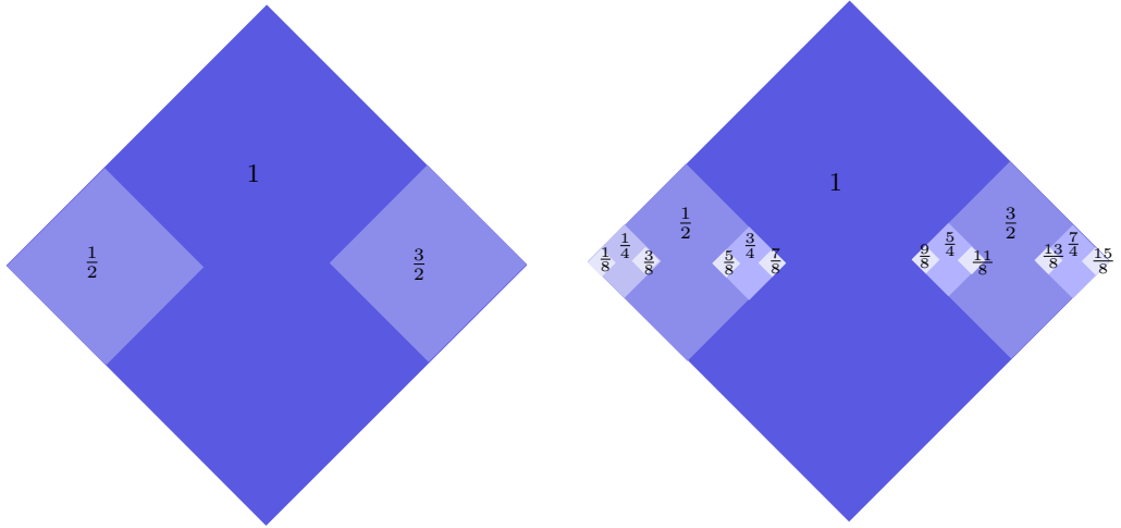
FIGURE 1.6. The functions u_2 and u_4 in the construction of Example 1.22.
