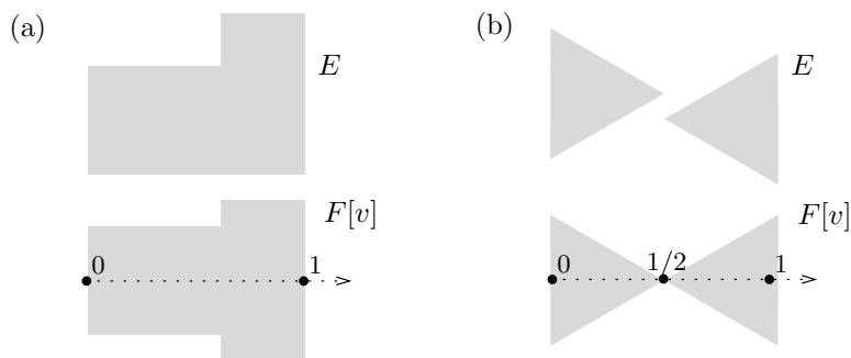
FIGURE 1.1. In case (a), \partial^* F[v] has vertical parts over \Omega = (0, 1) and (1.6) does not hold; in case (b), \partial^* F[v] has no vertical parts over \Omega = (0, 1) , but (1.5) fails (indeed, 0 = v^\vee(1/2) = v^\wedge(1/2) ).
