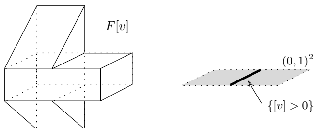
FIGURE 1.2. A polyhedron in \mathbb{R}^3 such that the rigidity condition (1.6) holds (with \Omega = (0, 1)^2 ) but the “no vertical parts” condition fails.
