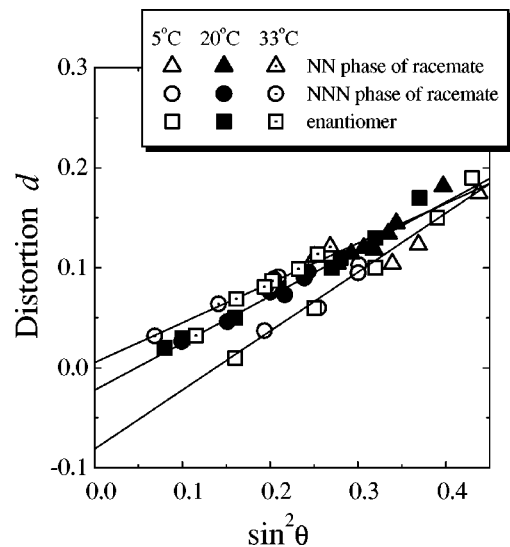
FIG. 4. The unit cell distortions versus \sin^2 \theta at different temperatures for racemic and enantiomeric monolayers.
