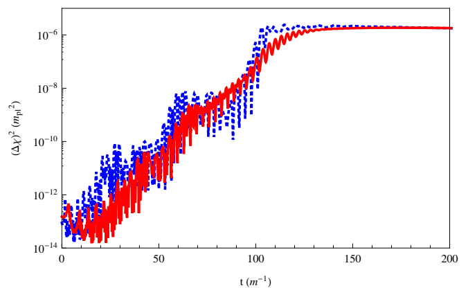
FIG. 2. Variance of the matter \chi fields. The red (solid) lines represent the fields when \lambda/\mu^4 = 5000 (initial \gamma = 8.7 ), and the blue (dotted) lines represent the canonical ( f \rightarrow 0 ) case.
