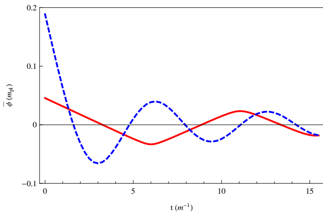
FIG. 1. Evolution of the mean inflaton field value for simulations with \lambda/\mu^4 = 5000 , \gamma_0 \approx 8.7 (red solid line) and the canonical case f \rightarrow 0 (blue dashed line).
