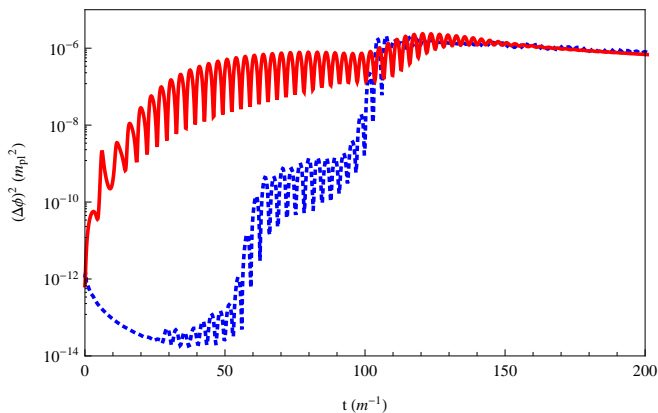
FIG. 3. Variance of the inflaton \phi field. The red (solid) lines represent the fields when \lambda/\mu^4 = 5000 (initial \gamma = 8.7 ), whereas the blue (dotted) lines represent the canonical ( f \rightarrow 0 ) case.
