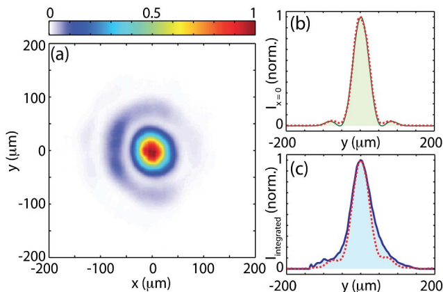
Fig. 2. (a) THz beam profile recorded via the proposed nonlinear imaging technique. (b) Section of the THz beam along the y coordinate ( x = 0 ) overlapped with a Bessel-Gauss beam fit (green, shaded). (c) Measured profile integrated on the x direction compared to the result of a knife-edge measurement (blue, shaded).
