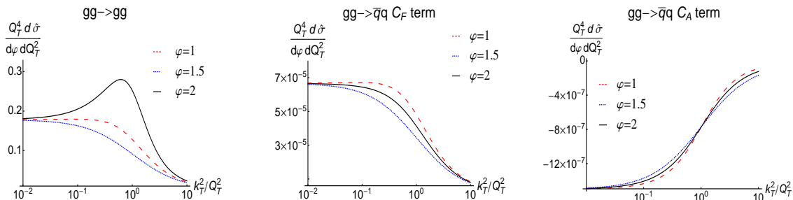
Figure 6. The k_T/Q_T dependence of the factorizing gg matrix elements: (a) gg \rightarrow gg ; (b) gg \rightarrow q\bar{q} C_F term; (c) gg \rightarrow q\bar{q} C_A term ( \xi_1\xi_2 S/Q_T^2 = 10^2 , \alpha_s = 0.2 ).
