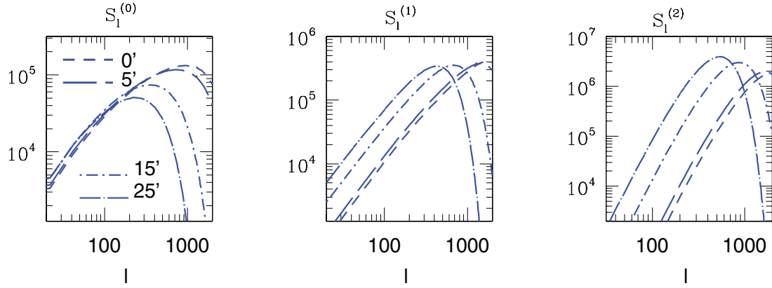
Figure 3. The absolute values of skew-spectra are plotted as a function of the harmonic l . From left to right the plots correspond to S_l^{(0)} , S_l^{(1)} and S_l^{(2)} , respectively. We consider four different beams with FWHM = 0, 5, 15 and 25 arcmin, respectively, as indicated. These results correspond to ideal noise-free experiments, and the resolution is taken to be l_{\max} = 2000 . The results are obtained using halo model prescription.
