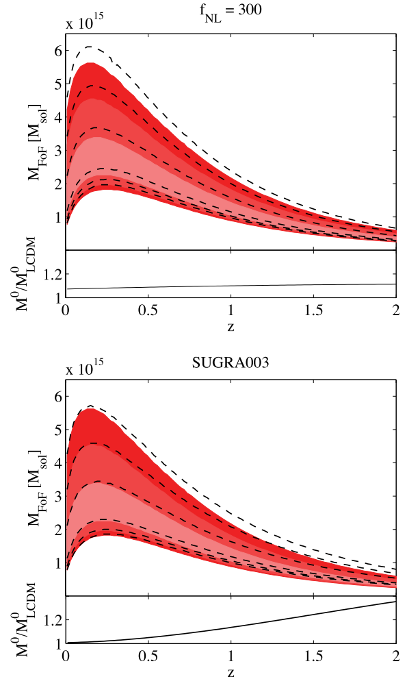
Figure 2. Extreme value contours for \Lambda CDM (shaded regions), f_{\text{NL}} and SUGRA models (dashed lines). Lower plots are the enhancement of modal highest mass cluster over the \Lambda CDM value, showing different behaviour for the two alternative models.
