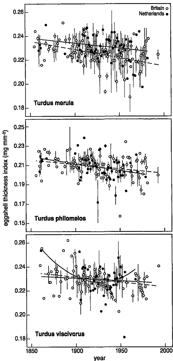
Fig. 1 Relationship between annual mean eggshell thickness index ( \text{mg mm}^{-2} ) ( \pm SE) and year of collection for British (o) and Dutch (●) Blackbird Turdus merula , Song Thrush T. philomelos , and Mistle Thrush T. viscivorus . Weighted regression lines for year shown for Dutch (—) and British (---) data; for full models see Table 1. For Mistle Thrush the weighted regression lines for both linear and quadratic effect of year are shown. British data from Green (1998).
