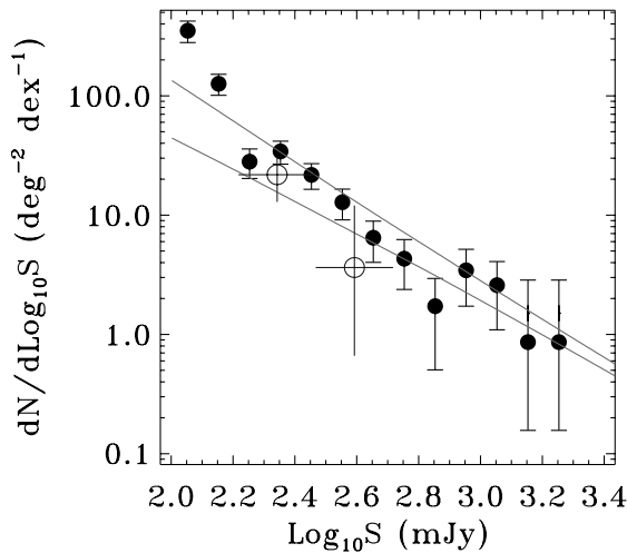
Figure 3. ELAIS source counts at 90 \mu\text{m} , compared with a no-evolution model (shallow curve) and the (1+z)^3 luminosity evolution model (steeper curve). The no-evolution curve has a slightly shallower slope than its Euclidean equivalent. Also shown as open symbols are the Lockman Hole counts from Linden-Vørnle et al. (2000). All errors are Poissonian, except in the case of a single object in a bin for which the \pm 1\sigma bounds on the number of objects in the bin are 0.18–3.3.
