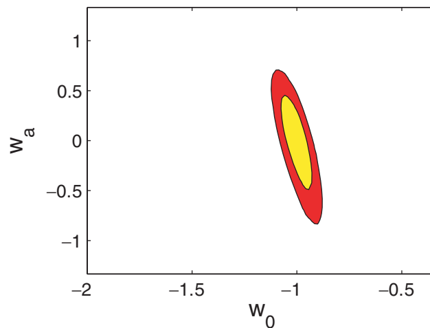
Figure 2. This plot shows a parameter error forecast for the SNAP SN Ia experiment, taking \Lambda CDM as the true model. The contour levels indicate 68 and 95 per cent. While this figure uses the full likelihood, in this case a Gaussian approximation using the Fisher matrix gives essentially identical results.
