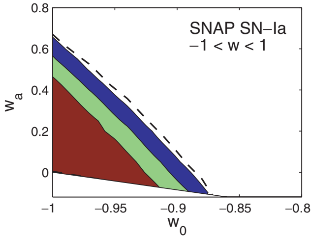
Figure 5. SNAP Bayes' factor contours for the quintessence prior on w_0 and w_a . The lower left-hand region is cut-off by the prior. The dashed contour shows the location of the \ln B_{01} = -5 contour for our full prior, as given in Fig. 1.
