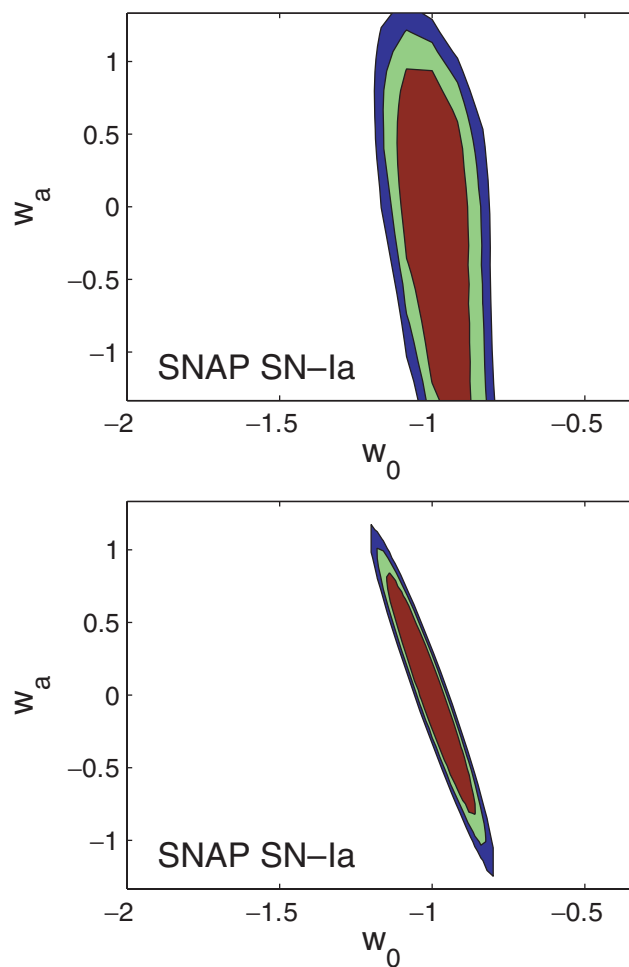
Figure 4. Bayes’ factor forecasts for SNAP assuming different external knowledge of \Omega_m . Contours are again shown for \log(B_{01}) > 0 , -2.5 and -5 . A Gaussian external constraint on \Omega_m is assumed, of width 0.03 (top panel) reflecting approximately the current level of uncertainty on it, and 0.003 (lower panel) reflecting an optimistic outcome.
