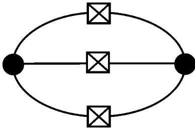
FIG. 1. The integrand of the nonstandard term in Eq. (17). The two vertices S^{(3)} are denoted by \bullet , the six internal lines are the propagators G=(S^{(2)}+k'^2)^{-1} , and the three insertions correspond to k'^2 .
