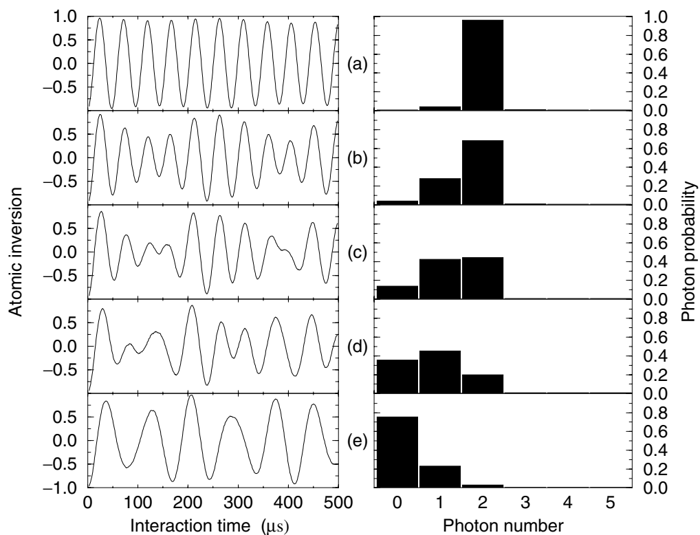
Figure 9. This figure shows Rabi oscillations (left) experienced by a probe atom at various time intervals after the creation of a two-photon Fock state. After creation and in the presence of dissipation, the Fock state decays (right) finally ending up in the ground state after a long time delay. If this was a classical decay, the frequency of the Rabi oscillations would smoothly vary from top (a) to bottom (e). This is pictured in figure 10. Quantum mechanical decay, on the other hand, is dominated by the original Fock state for the initial portion of the decay (b), with the frequency of oscillation determined by equation (1).
