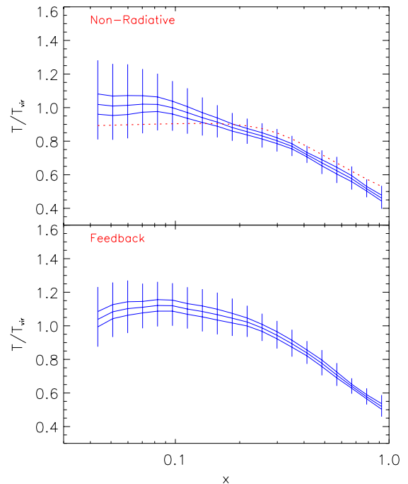
Figure 7. Dimensionless temperature profiles for clusters in the non-radiative and feedback models. The best-fitting profile to the results of Rasia et al. (2004) is shown as a dotted curve.
