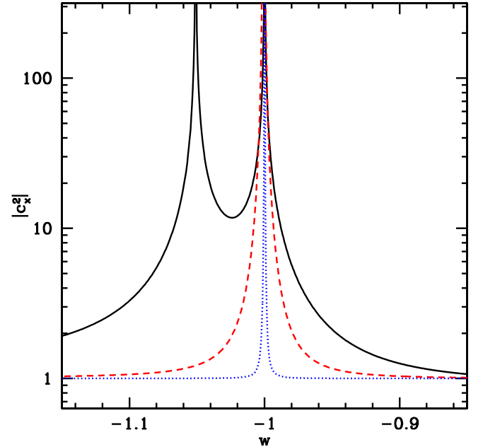
FIG. 7 (color online). We plot the apparent sound speed c_x^2 defined by Eq. (58) for three different wave vectors, k = 1/H_0 (black solid line), k = 10/H_0 (red dashed line), and 100/H_0 (blue dotted line). Although the real sound speed is just \hat{c}_s^2 = 1 , the apparent sound speed diverges at w = -1 and can even become negative.
