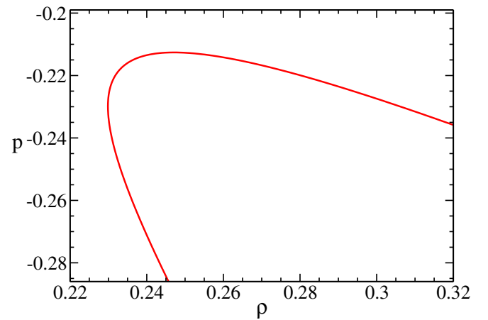
FIG. 2 (color online). The pressure as a function of the energy density. The graph of p(\rho) shows that p is not a single valued function of the energy density, and that there is a point with an infinite slope (corresponding to the minimum of \rho and the divergence of c_a^2 ). The point where p(\rho) has a zero slope corresponds to the maximum of p and a vanishing c_a^2 .
