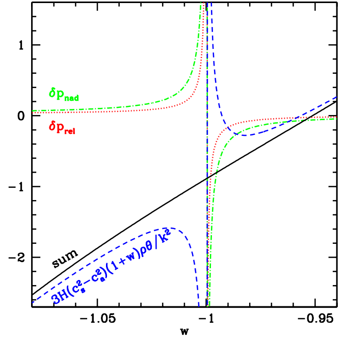
FIG. 6 (color online). This figure shows the different divergent contributions to the pressure perturbation, Eq. (54), multiplied by 10^9 . The relative pressure perturbation is shown as red dotted lines, the nonadiabatic pressure perturbation as green dash-dotted lines and the contribution from the gauge transformation to the conformal Newtonian frame as blue dashed lines. Each of the contributions diverges at the phantom crossing, but their sum (shown as black solid line), and so \delta p , stays finite.
