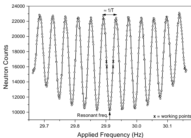
FIG. 2. The Ramsey resonance curve for spin-up neutrons, N_{\uparrow} . The corresponding pattern for N_{\downarrow} is inverted but otherwise identical.
