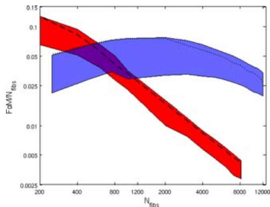
Figure 7. Constructed from the same data as Fig. 6, but we now plot FoM/ n_{\text{fibres}} against the number of fibres, to find the most efficient use of the instrument.
