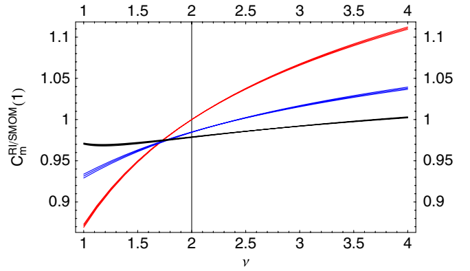
FIG. 4 (color online). Residual matching-scale dependence of the conversion factor C_m^{\text{RI}/\text{SMOM}} at \omega = 1 at LO (red), NLO (blue), and NNLO (black).
