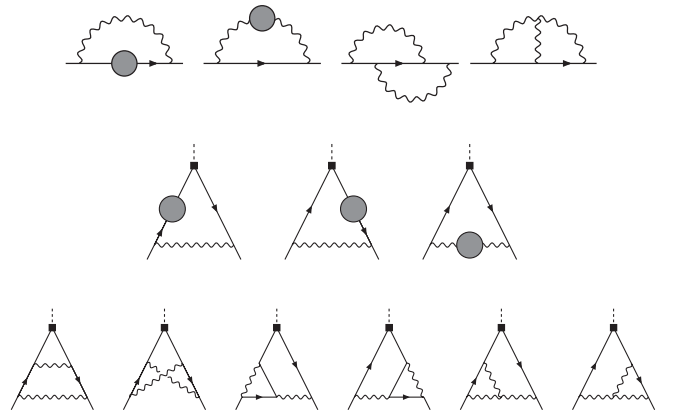
FIG. 1. Two-loop propagator and vertex diagrams. The grey blobs indicate a sum over all one-loop corrections to a propagator; the black boxes indicate an insertion of a fermion bilinear.
