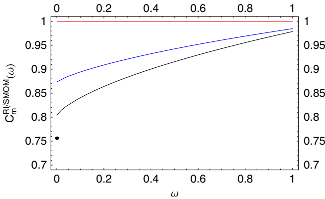
FIG. 3 (color online). Conversion factors C_m^{\text{RI}/\text{SMOM}} as function of \omega = q^2/p^2 at LO (top/red), NLO (middle/blue), and NNLO (bottom/black), and C_m^{\text{RI}/\text{MOM}} = C_m^{\text{RI}/\text{SMOM}}(0) at NNNLO (dot).
