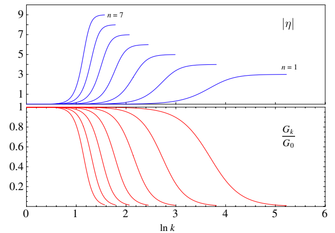
FIG. 1 (color online). Running anomalous dimensions (upper panel) and gravitational couplings (lower panel) from (5) and (6) for D = 4 + n dimensions with n = 1, \dots, 7 (from right to left). The crossover takes place at the respective Planck scale.
