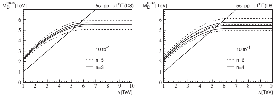
FIG. 2. The 5\sigma discovery contours in M_D at the LHC, shown as a function of a cutoff \Lambda on E_{\text{parton}} for an assumed integrated luminosity of 10 \text{ fb}^{-1} . Thin lines show a \pm 10\% variation of k_{\text{tr}} about M_D , the straight line is M_D^{\text{max}} = \Lambda . The leveling off at M_D^{\text{max}} \approx \Lambda reflects the gravitational UV fixed point. To enhance the reach we require m_{\ell\ell}^{\text{min}} = \min(M_D/3, 2 \text{ TeV}) .
