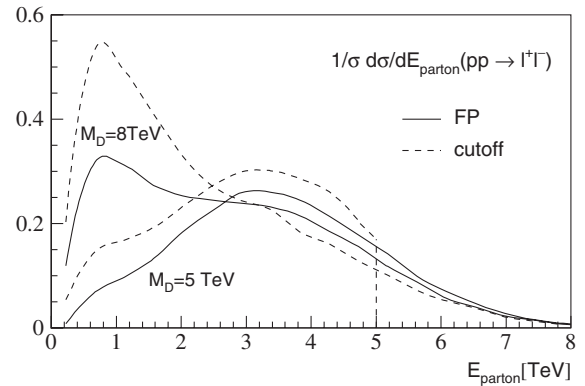
FIG. 3. Comparison of normalized distributions of the partonic energy E_{\text{parton}} for the dimension-8 operator correction to Drell-Yan production at the LHC ( n = 3 ). Full line: present work, dashed line: approximation (9) with \Lambda = M_D .
