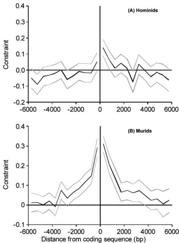
Figure 1. Selective Constraint Plotted against Distance from the Coding Sequence in 5' Flanking Regions and 3' Flanking Regions
