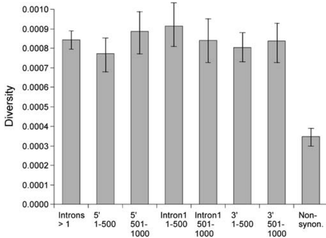
Figure 3. Mean Nucleotide Diversity in Human Intergenic DNA in Blocks of 500 Bases Upstream and Downstream of Genes
