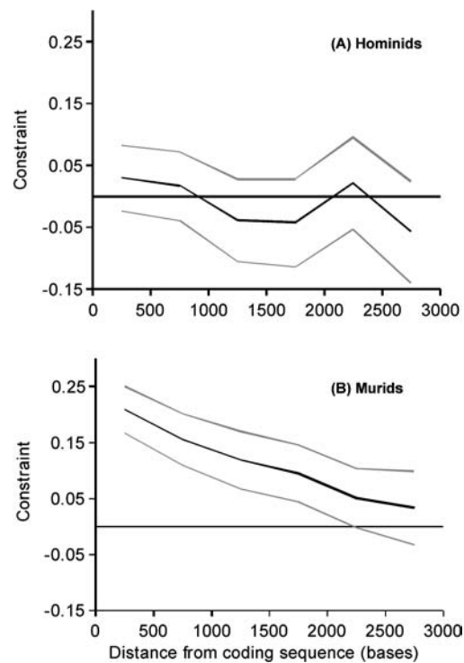
Figure 2. Selective Constraint at the 5' End of First Introns Plotted against Distance from the Intron Start
