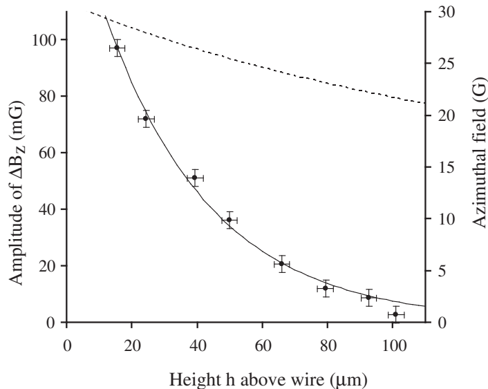
Figure 4. Magnetic fields versus height h above a wire carrying 3.7 A. Data points: amplitude of the anomalous magnetic field variation \Delta B_z . Solid line: best fit of the modified Bessel function aK_1(2\pi(h + \delta)/\lambda) . This has \lambda = 217 \pm 10 \mu\text{m} and \delta = 251 \pm 12 \mu\text{m} . Dashed line: The (usual) azimuthal field referred to the auxiliary ordinate on the right.
