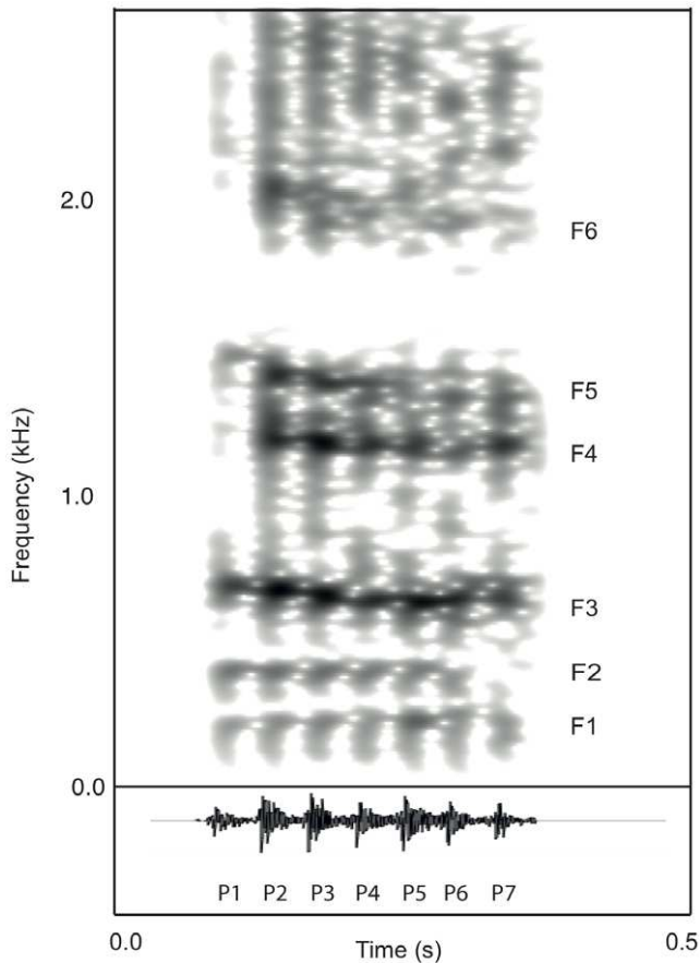
Figure 2. Spectrogram (A) and waveform (B) of a male fallow deer groan. Male fallow deer groans are low-pitched vocalisations characterised by a rapid downward shift in formant frequencies across the call (spectrogram settings: FFT method, window length=0.05 s, time step=0.01 s, Gaussian window shape, dynamic range=30 dB). doi:10.1371/journal.pone.0021066.g002
