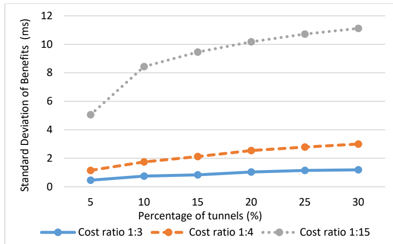
Figure 4 Standard Deviation of Cost Benefit for different cost ratio
