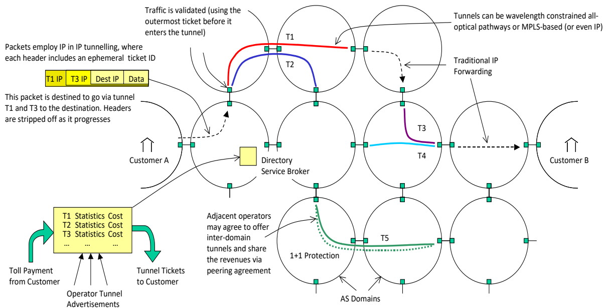
Figure 1 User-Selectable AS Domain Tunnelling Framework
