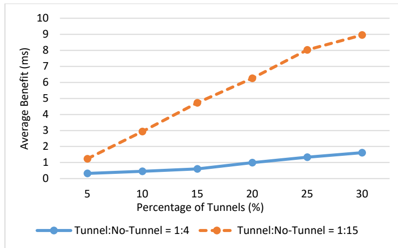
Figure 5 Average of Cost Benefit for different cost ratio
