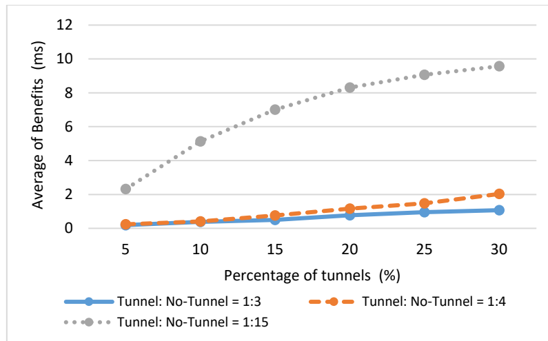
Figure 3 Average of Cost Benefit for different cost ratio
