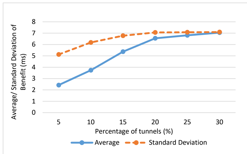
Figure 6 Average and Standard deviation of Cost Benefit for Tunnel-No Tunnel = 1:15
