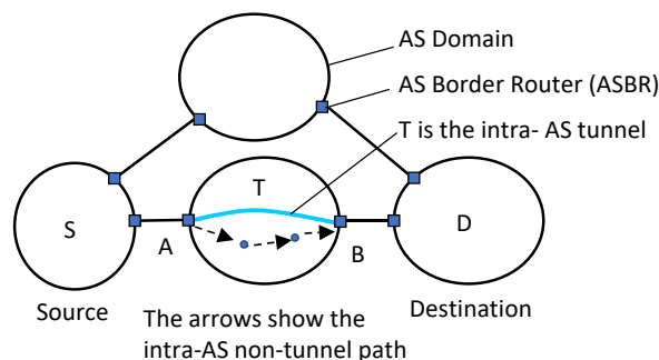
Figure 2 Example Intra-AS path with and without Tunnels
