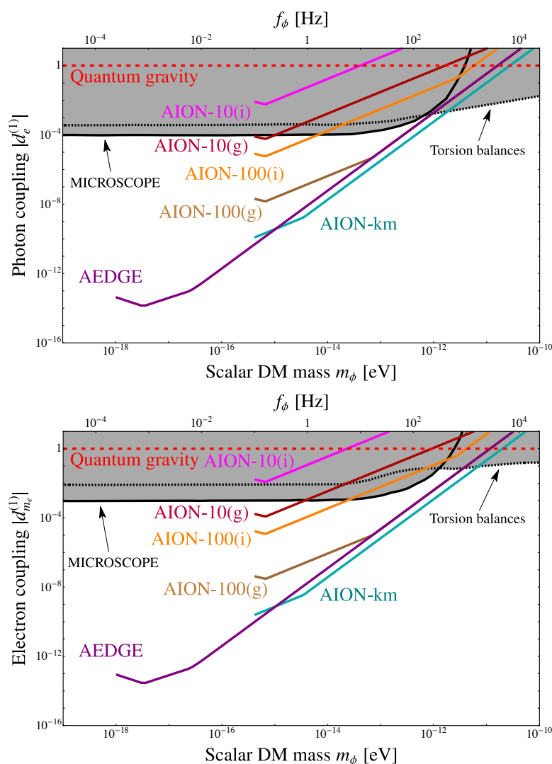
Figure 1. Bounds on the parameters d_e^{(1)}, d_{m_e}^{(1)} as a function of the mass of the scalar field. Quantum gravity predicts d_e^{(1)}, d_{m_e}^{(1)} \sim 1 , closing all of the parameter space accessible to atom interferometers. Note initial (i) and goal (g) sensitivities for AION are displayed.
