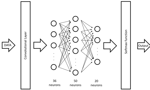
Fig. 4. Behavior identification neural network
