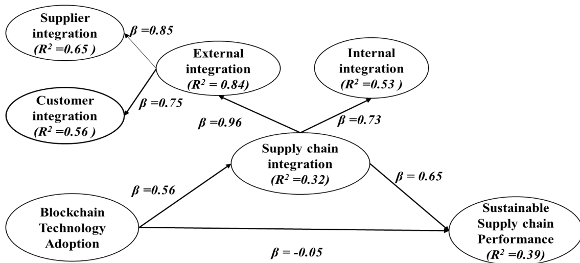
Figure 2: Integrated structural equation model
